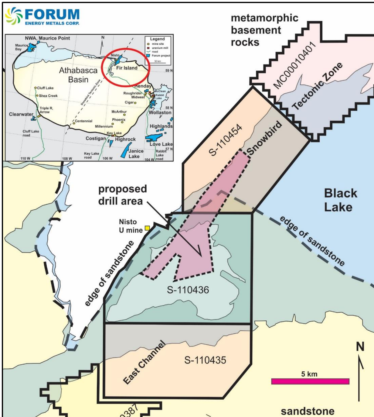
Figure 1: Fir Island Location Map. The project lies along the northern contact of the Athabasca sandstone and is transected by the major Snowbird Tectonic Zone, which offsets the sandstone approximately 10km to the north.
