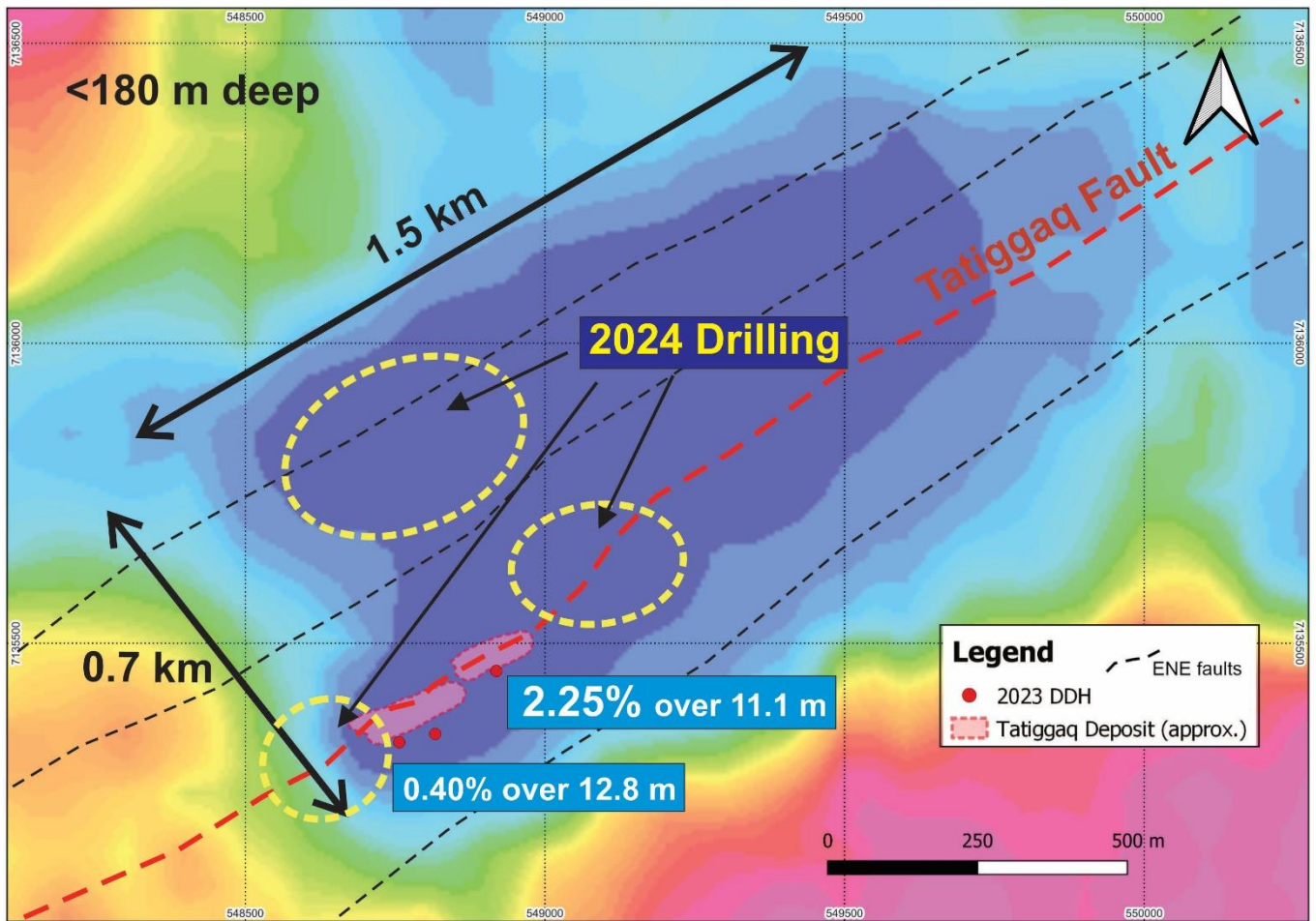
Figure 3 Tatiggaq gravity anomaly, 2023 drill holes and 2024 Phase One drilling to the west-southwest and the east-northeast along the Tatiggaq Fault. Ambient Noise Tomography (ANT) modelled sub-parallel east-northeast-trending faults have also been targeted.
