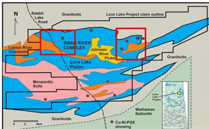
Figure 1 - Geology Map of the Love Lake Pluton. Claim outline is shown in black, red outlines show areas where work will be completed for this program
