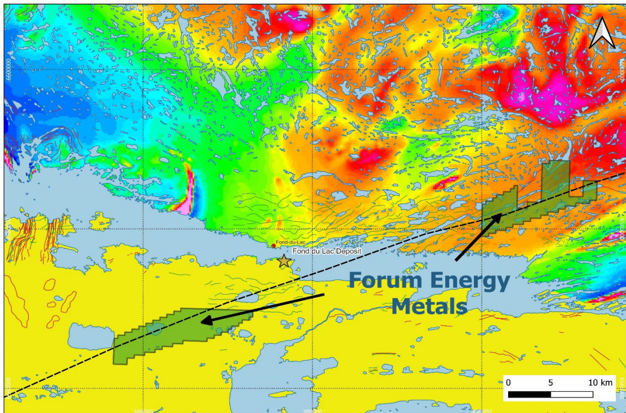
Figure 1. Location of the Grease River Project in northern Saskatchewan nearby the community of Fond-du-Lac. The southern claim block is in Athabasca Basin sandstone cover (yellow) and the northern block is in basement rocks (shown with background magnetics). Dashed line is the Grease River Shear Zone.
